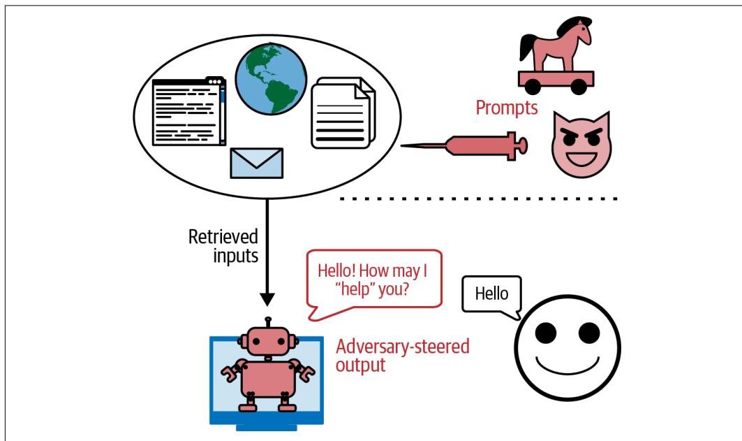
Figure 5-12. Attackers can inject malicious prompts and code that your model can retrieve and execute. Image adapted from “Not What You’ve Signed Up for: Compromising Real-World LLM-Integrated Applications with Indirect Prompt Injection” (Greshake et al., 2023).
